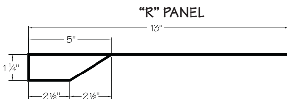
Wall-to-Roof Flashing
